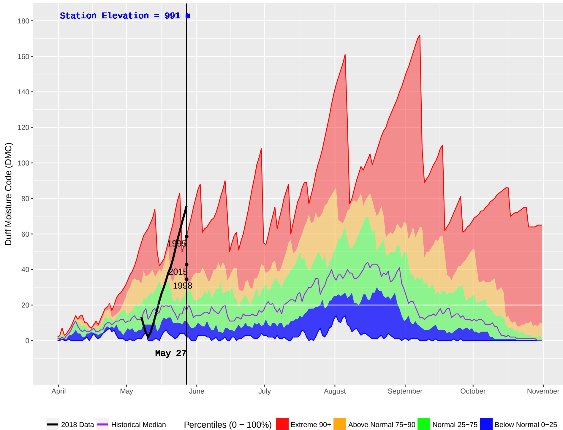
TROUT LAKE (387) : Historical (1987–2016) and Current (2018) Noon Duff Moisture Code (DMC)
